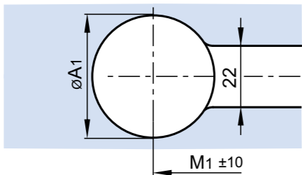
8-12SMT/-DMT View: Recess in the frame plate
