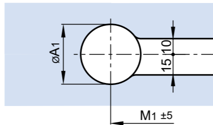
5SMTK/-DMTK View: Recess in the frame plate
