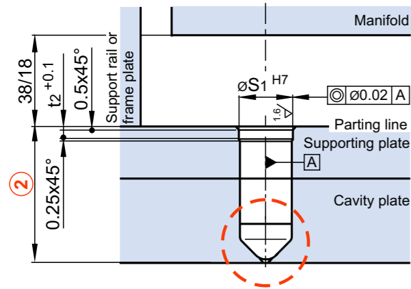
4-6SMT/-DMT View: Recess in the frame plate
