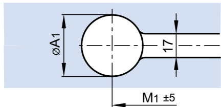
4-6SMT/-DMT View: Recess in the frame plate
