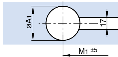
View: Recess in the frame plate
