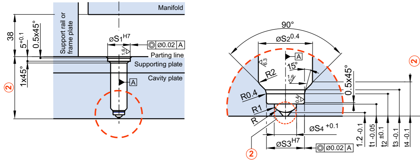
View: Recess in the frame plate
