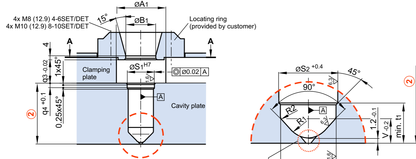
View A-A: Clamping plate
