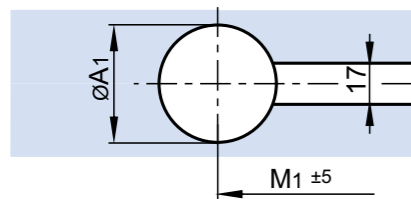
View A-A: Recess in the frame plate
